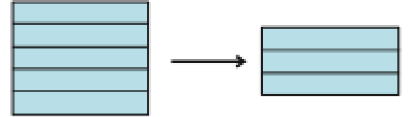
Discretization
